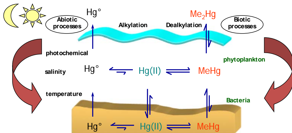
Hg Geochemical Cycle
