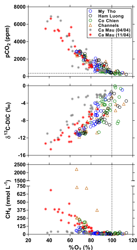
Figure 10. Distribution as a function of oxygen saturation level (%O 2 , %) of the partial pressure of CO 2 (pCO 2 , ppm), stable isotope composition of dissolved inorganic carbon ( \delta^{13}\text{C-DIC} , ‰), and dissolved CH 4 concentration ( \text{nmol L}^{-1} ) in the three branches of the Mekong delta (Mỹ Tho, Hàm Luông, and Cỏ Chiên) and side channels and in the mangrove creeks of the Ca Mau province in April and October 2004. The vertical dotted line indicates O 2 saturation (100 %); the horizontal line indicates the average atmospheric pCO 2 value.
