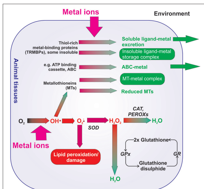
FIGURE 3 | Simplified synthesis of the routes of metal toxicity and detoxification in animal tissues. Metals in the environment that enter animal tissues can be sequestered by various metal binding proteins, including metallothioneins and other thiol-rich peptides, and either stored or excreted from those tissues. Metallothioneins can also detoxify hydroxyl radicals within cells. Redox active metals can drive the formation of superoxide anions ( O_2^{\bullet-} ) via hydroxyl radicals ( OH^{\bullet} ) that, if unregulated, can lead to lipid peroxidation and damage to cellular membranes. Superoxides can be enzymatically converted to hydrogen peroxide by superoxide dismutase (SOD). Hydrogen peroxide ( H_2O_2 ) is enzymatically converted to water by catalases and peroxidases (CAT and PEROXs, respectively) or by the action of glutathione peroxidase (GPx) and glutathione disulphide reductase (GR). Synthesis adapted from: Stocker and Keaney (2004), Aitken and Roman (2008), and Martinez-Finley and Aschner (2011).
