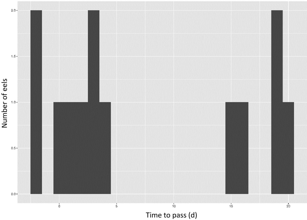
Fig. 4. Number of European eels and the time required to pass dam A. Time to pass is defined as the time difference between an individual first being detected in front of the dam, when the dam overflowed, and when the same individual was first detected downstream of the dam. Negative time to pass values indicate passage before overflowing, i.e., via the main pipe.
