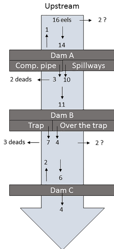
Fig. 3. Overview of the fates of tagged European eels for each dam.
