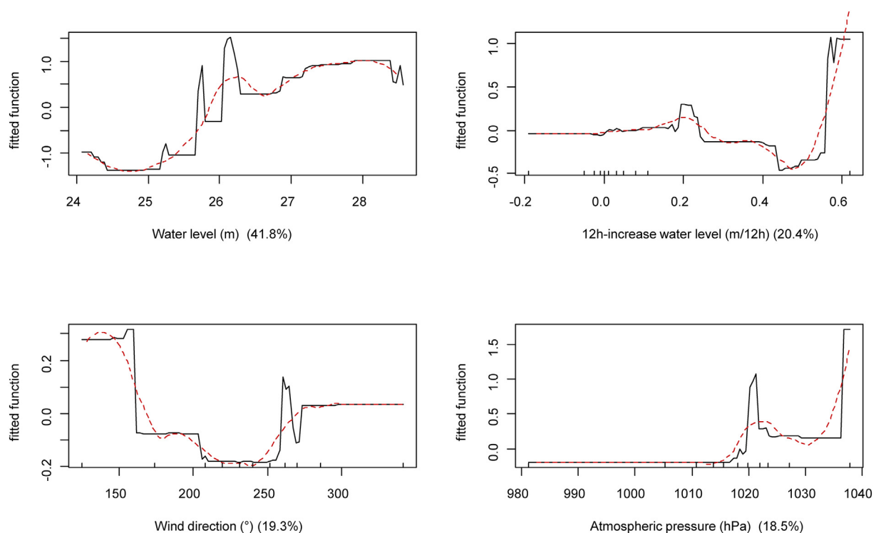
Fig. 2. Partial plots of the functions fitted for the final Boosted Regression Trees model describing the triggering of downstream movement. The relative contribution that explains the variance of each descriptor is shown in parentheses. Black lines represent raw data and red lines represent smoothed data. (For interpretation of the references to colour in this figure legend, the reader is referred to the web version of this article.)
