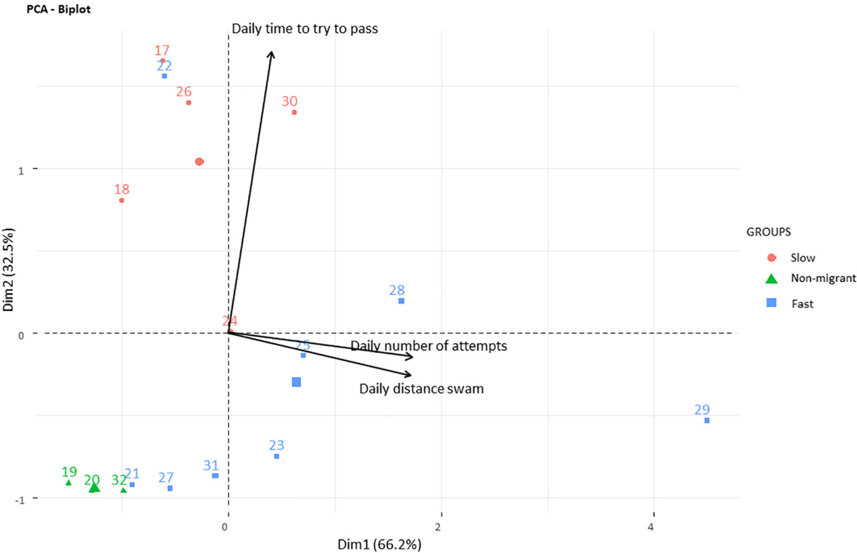
Fig. 5. Factorial map of the efficiency of individual European eels to pass through dam A based on behavioral metrics (indicated by arrows). Each eel is represented by a group symbol and a number, with a barycenter for each group.
