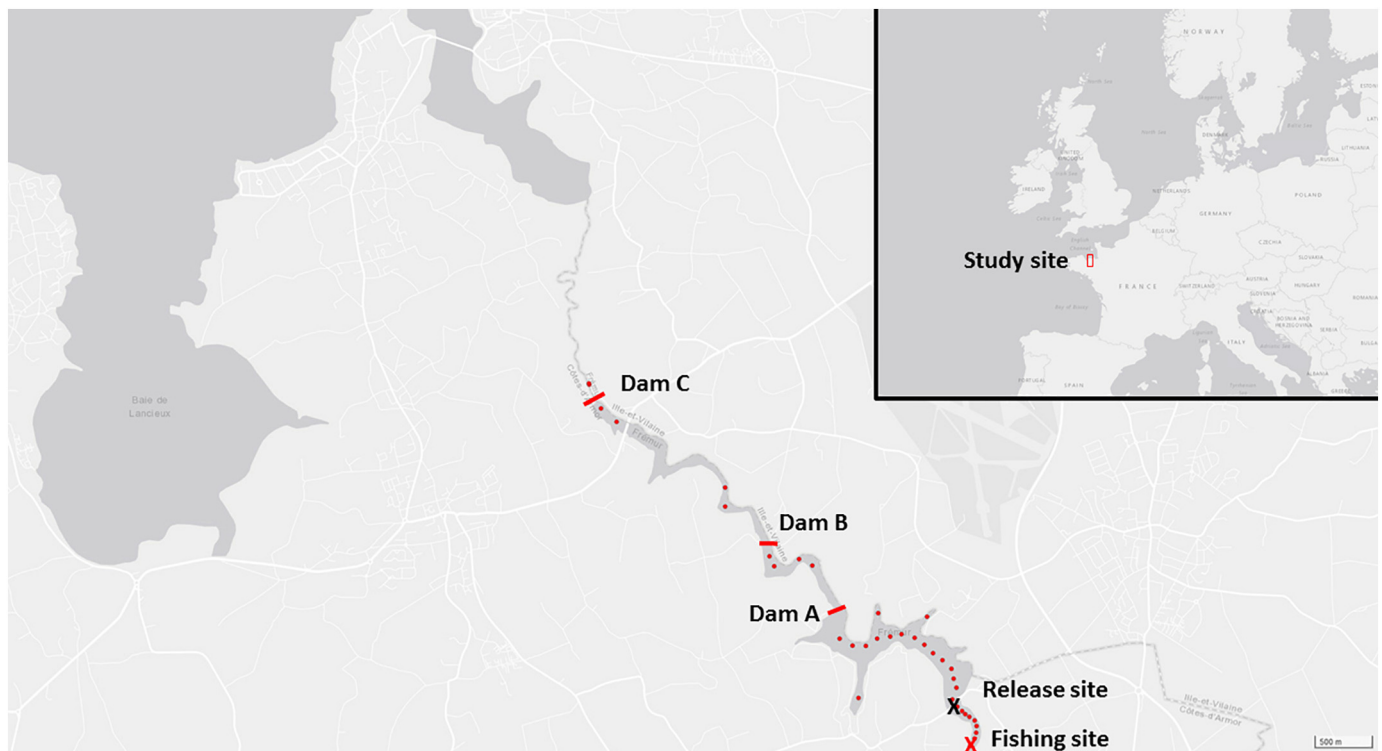
Fig. 1. Map indicating the positions of the acoustic receivers (red circles) in the Frémur River, northwestern France, and the A, B, and C dams. (For interpretation of the references to colour in this figure legend, the reader is referred to the web version of this article.)
